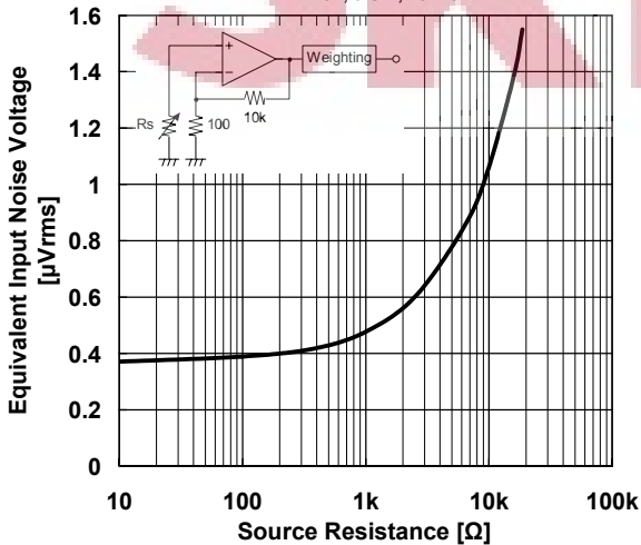
Voltage Noises vs. Source Resistance V^+/V^-=\pm 15V, JIS A, T_a=25^\circ C
